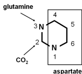
De novo synthesis of pyrimidines
