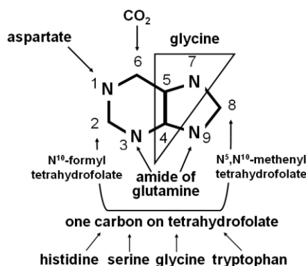
De novo synthesis of purines
