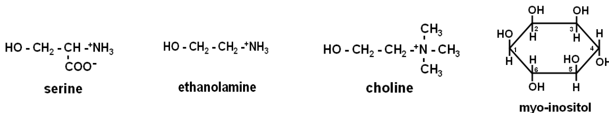
A typical glycerophospholipid
