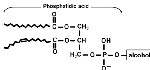
A typical glycerophospholipid
